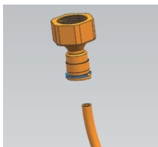
Step5) Make sure the end of the water piper insert into connector.
